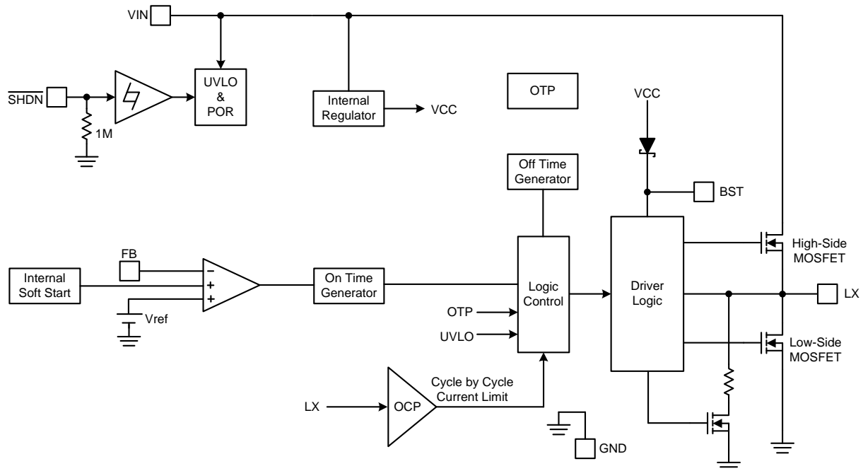
Figure 3. Block Diagram of FR9207
