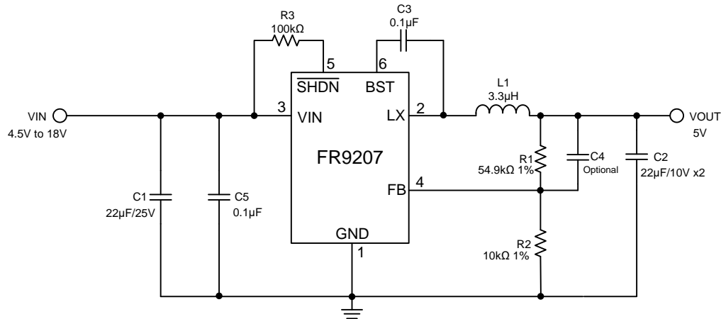
Figure 2. FR9207 Application Circuit
